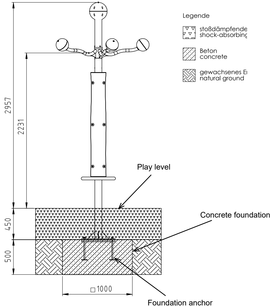
Diagram 2: Foundation plan
