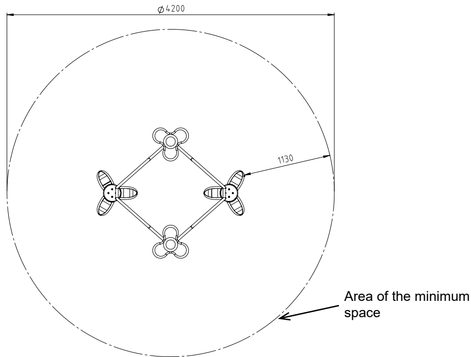
Diagram 3: Top view
