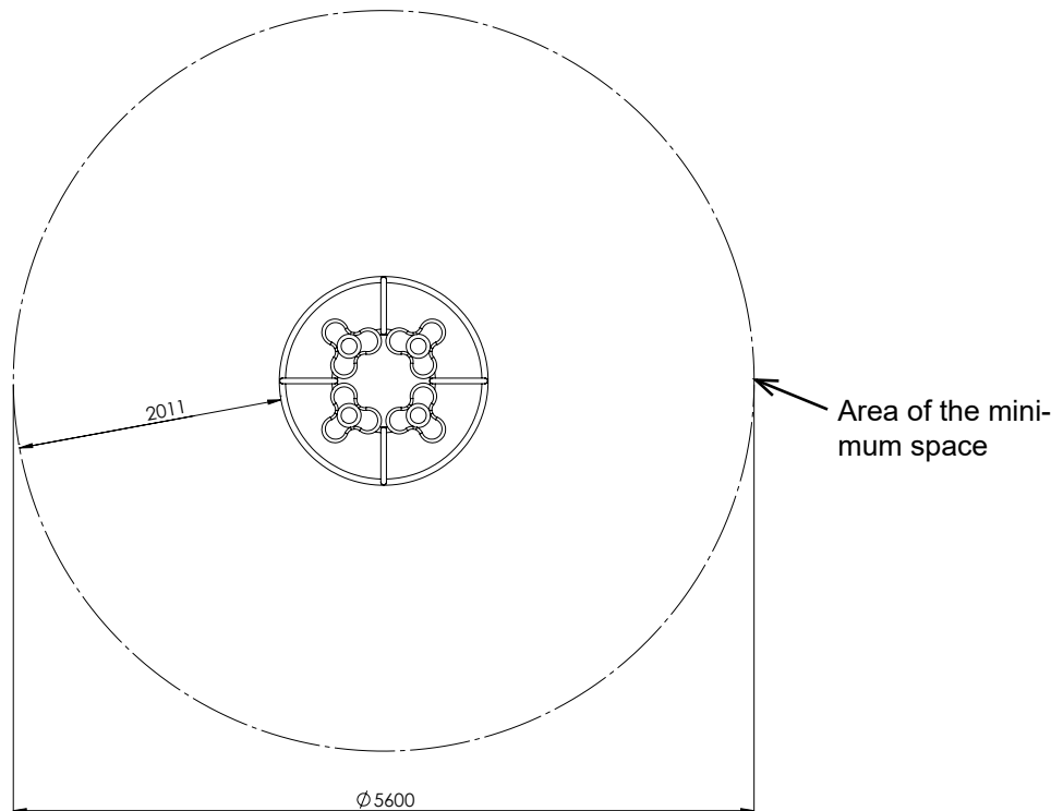
Diagram 3: Top view
