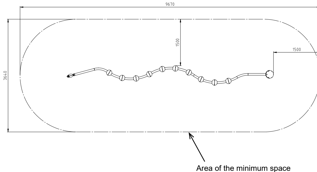
Diagram 3: Top view
