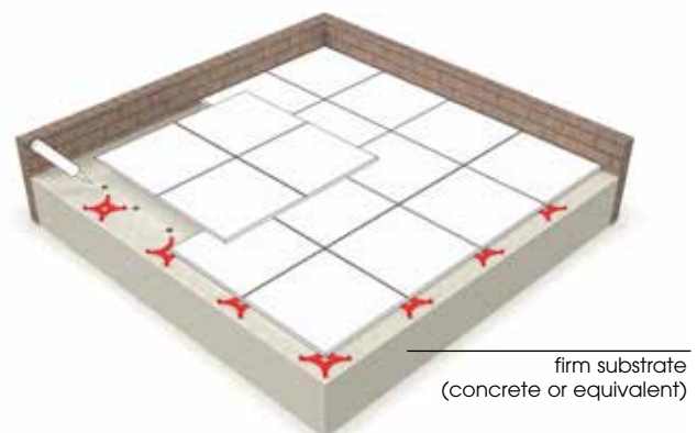
Laying of the Elastic Slab 30 with the Cross connector
